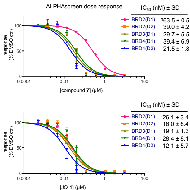
Figure 1. Dose response plots for AlphaScreen TM assays. Results of at least 2 independent experiments reported as mean ± SD.
