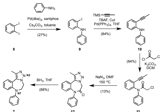
Scheme 1. Synthesis of 1,2,3-triazolobenzodiazepines: Synthesis of 7 .
