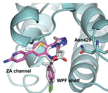
Figure 2. A X-ray crystal structure of 20 (magenta) in complex with BRD2(D2) PDB code = 5U6V overlaid with co-crystal structure of JQ-1 (grey) bound to BRD2(D2) PDB = 3ONI.
