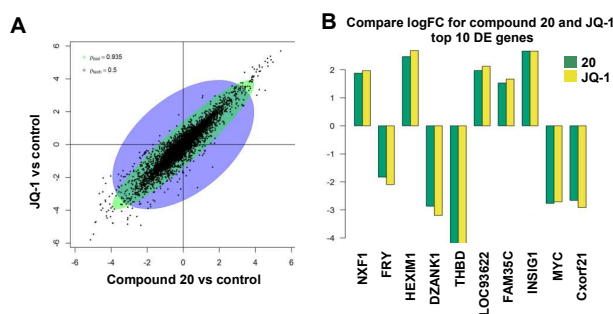
Figure 3. A. GENAS plot comparing effects of 20 and JQ-1 on THP-1 cells. B. Identity of 10 highest up and down regulated genes by 20 and JQ-1.
