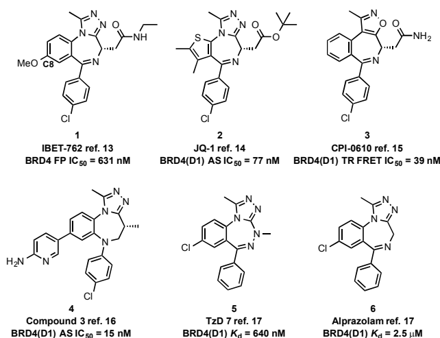
Chart 1. Example azepine BET inhibitors
