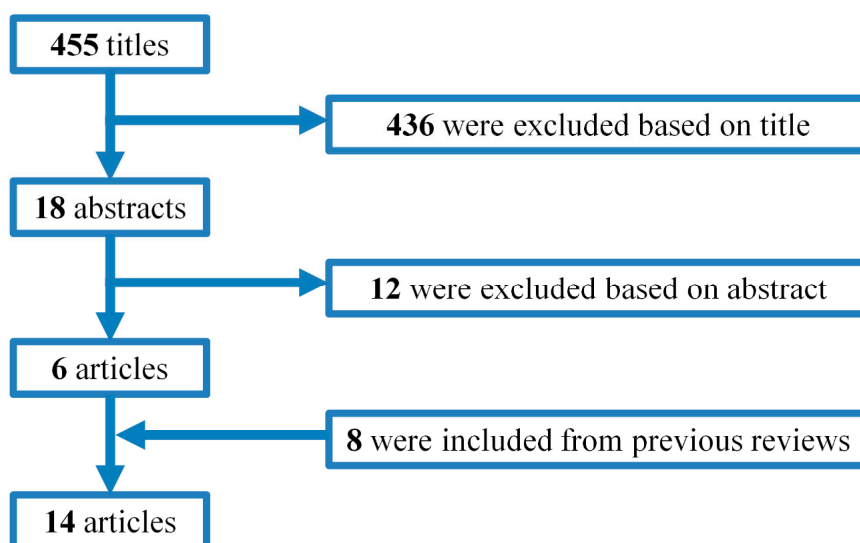
Figure 1. Study identification and selection.
