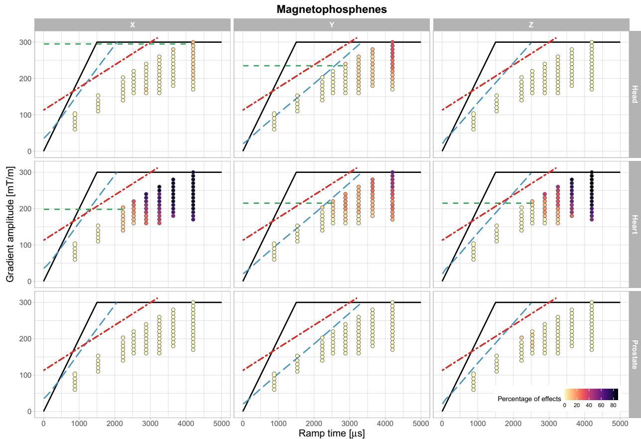
FIGURE 2 Percentage of participants reporting magnetophosphenes for the three imaging landmarks and three gradient axis. The dots are color-coded according to the percentage of volunteers reporting the effect for each of ramp time/gradient amplitude pair. The hardware limit (maximum slew rate and maximum gradient amplitude) is depicted as solid black line curve, the approximate location of the cardiac stimulation limit is shown as red dot-dashed line and the PNS limit (SAFE model, 33 for X, Y, and Z axes separately) is shown as blue dashed line. As outlined in the discussion, the magnetophosphene guideline value, G_{amp} , is shown as a green dashed line. This represents the maximum gradient amplitude, at the maximum slew rate, for which fewer than 10% of participants reported magnetophosphenes. This is not defined where the guideline value is greater than 300 mT/m
