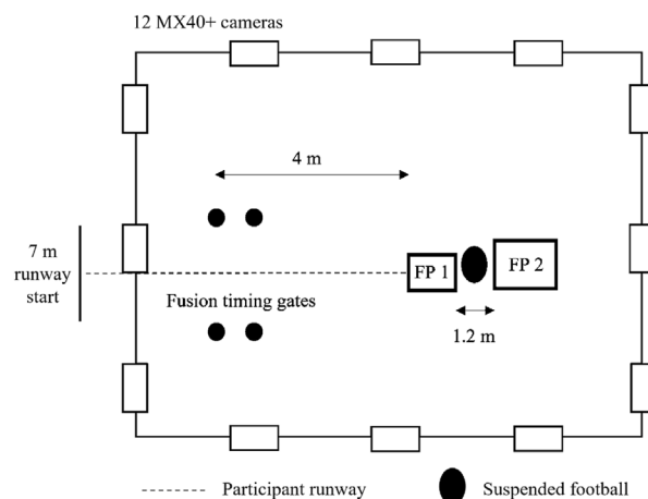
Fig. 1. Laboratory set-up for the running vertical jump test.
