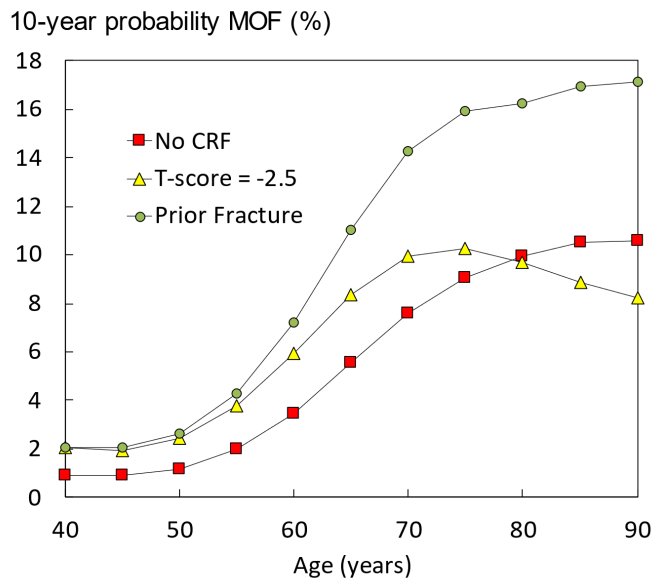
Fig. 1 10-year probabilities of a major osteoporotic fracture (MOF; hip, clinical spine, humerus and forearm) calculated with the Pakistani FRAX model for women.
